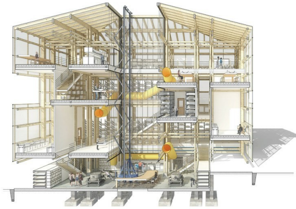
SECTION PERSPECTIVE
