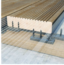
Fasteners for Wooden Decks and Facades Rothoblaas
